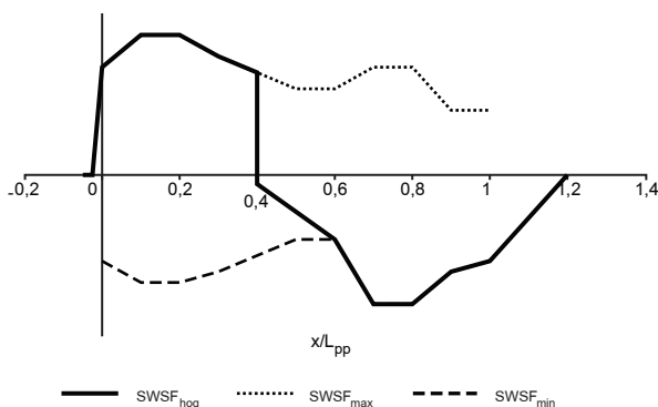
Figure 2 : Distribution of hogging still water shear force SWSF HOG
