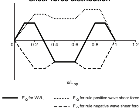
Figure 9 : Nondimensional negative amidship wave shear force distribution
