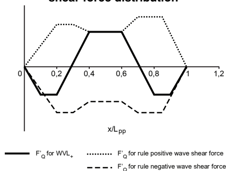
Figure 8 : Nondimensional positive amidship wave shear force distribution
