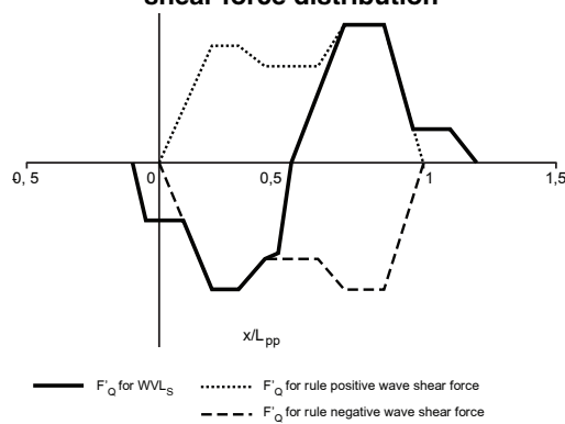
Figure 7 : Nondimensional sagging wave shear force distribution
