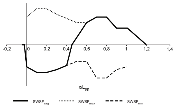
Figure 3 : Distribution of sagging still water shear force SWSF SAG
