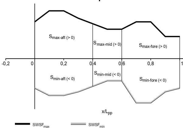
Figure 1 : Definition of areas from design still water shear force envelope distributions
