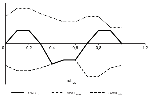
Figure 5 : Amidship negative still water shear force SWSF -
