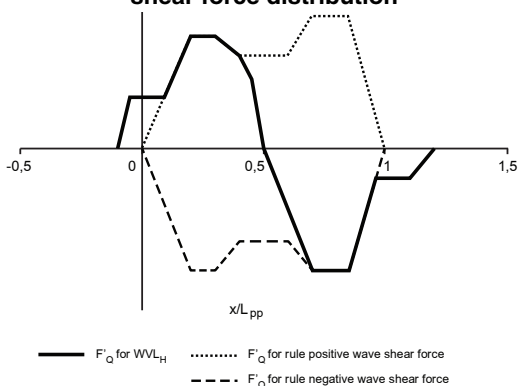
Figure 6 : Nondimensional hogging wave shear force distribution
