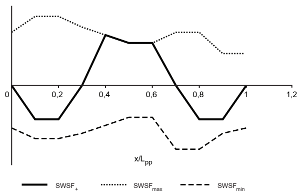
Figure 4 : Amidship positive still water shear force SWSF +
